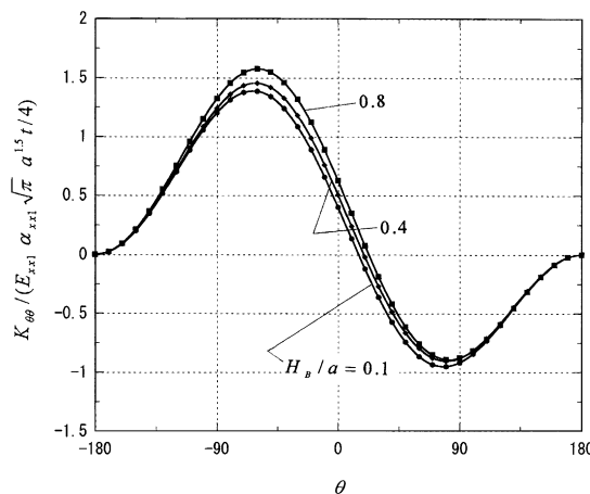
Fig. 8. Stress intensity factors K_{\theta\theta} versus \theta for H_B/a (=H_C/a) = 0.8, 0.4, 0.1 .
